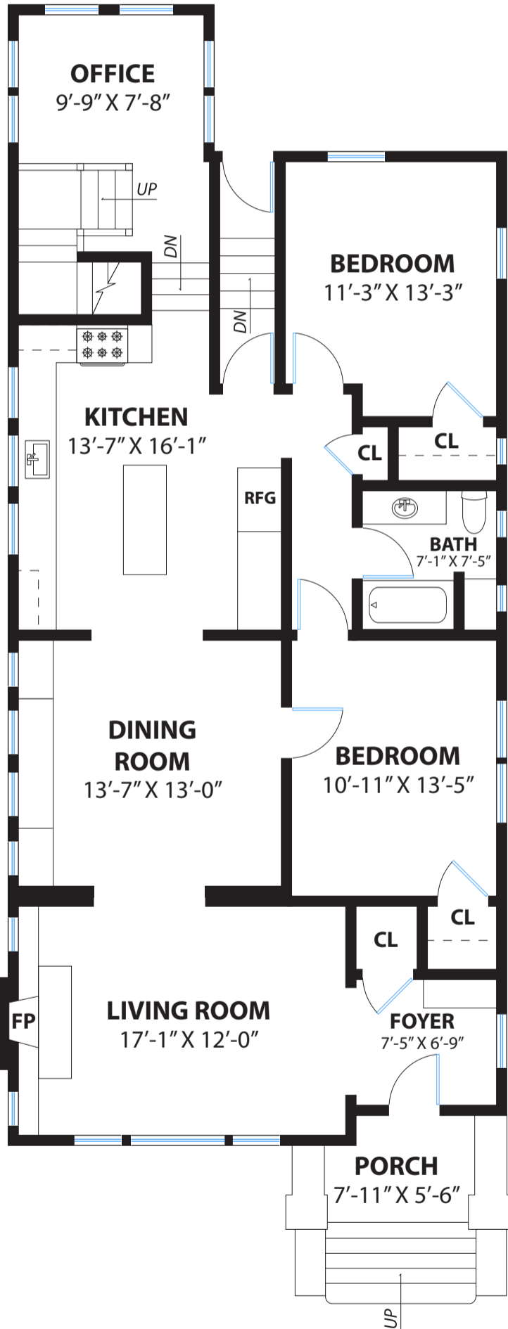
FIRST LEVEL
