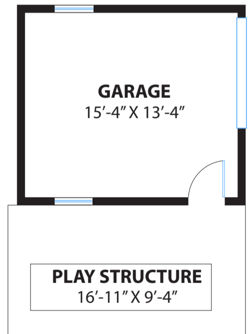
SECOND LEVEL
